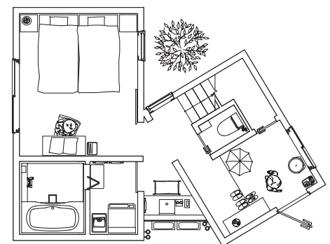
1F PLAN
